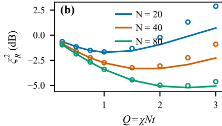
exact (circles) vs cumulant (lines)
