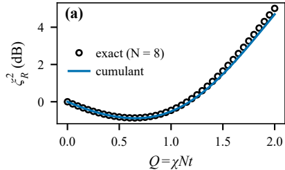
8 disordered spins, all noise channels
