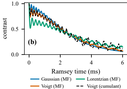
\chi N_0/2\pi = 7 kHz
