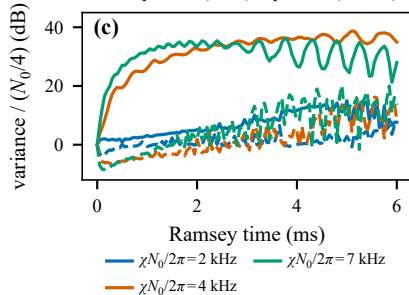
anti-squeezed (solid), squeezed (dashed)
