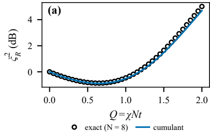
8 disordered spins, all noise channels
