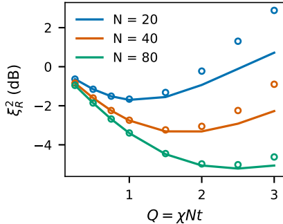
(b) Dicke exact (o) vs cumulant (-)
