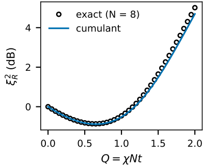
(a) disordered spins, all dissipators
