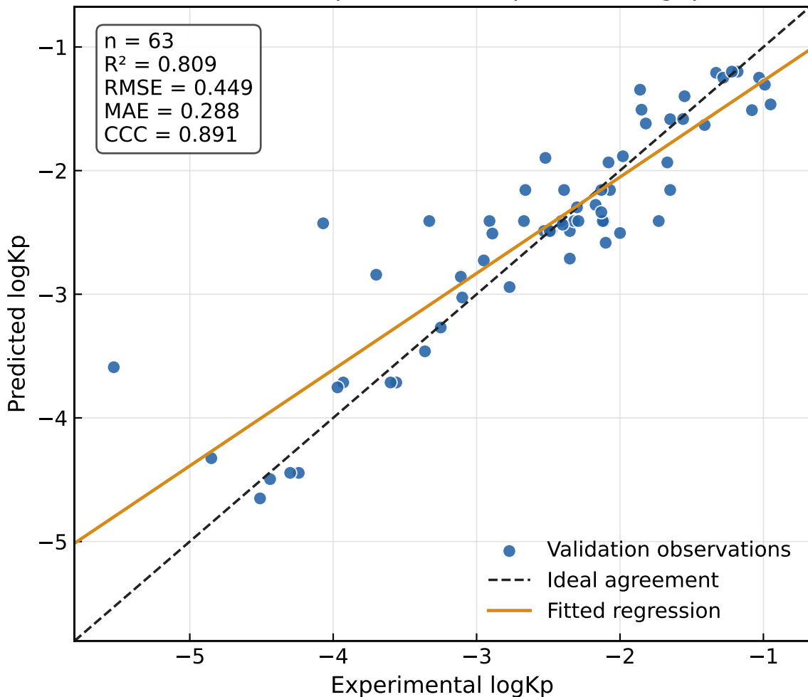
CatBoost: experimental vs predicted logKp
