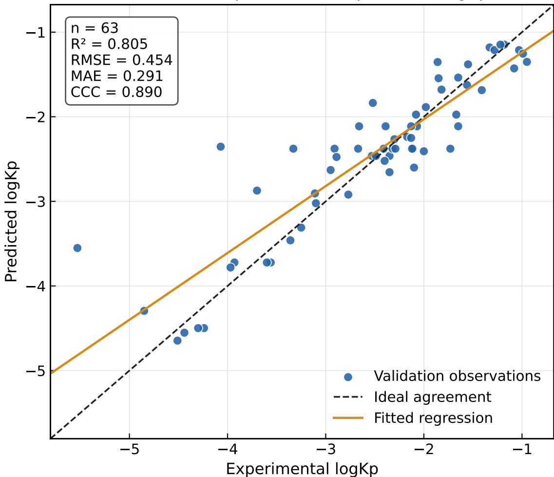
ExtraTrees: experimental vs predicted logKp
