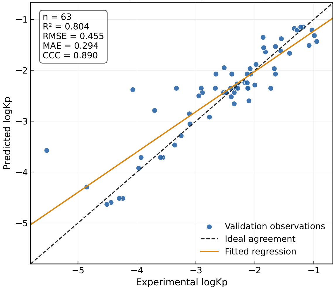
LGBM: experimental vs predicted logKp
