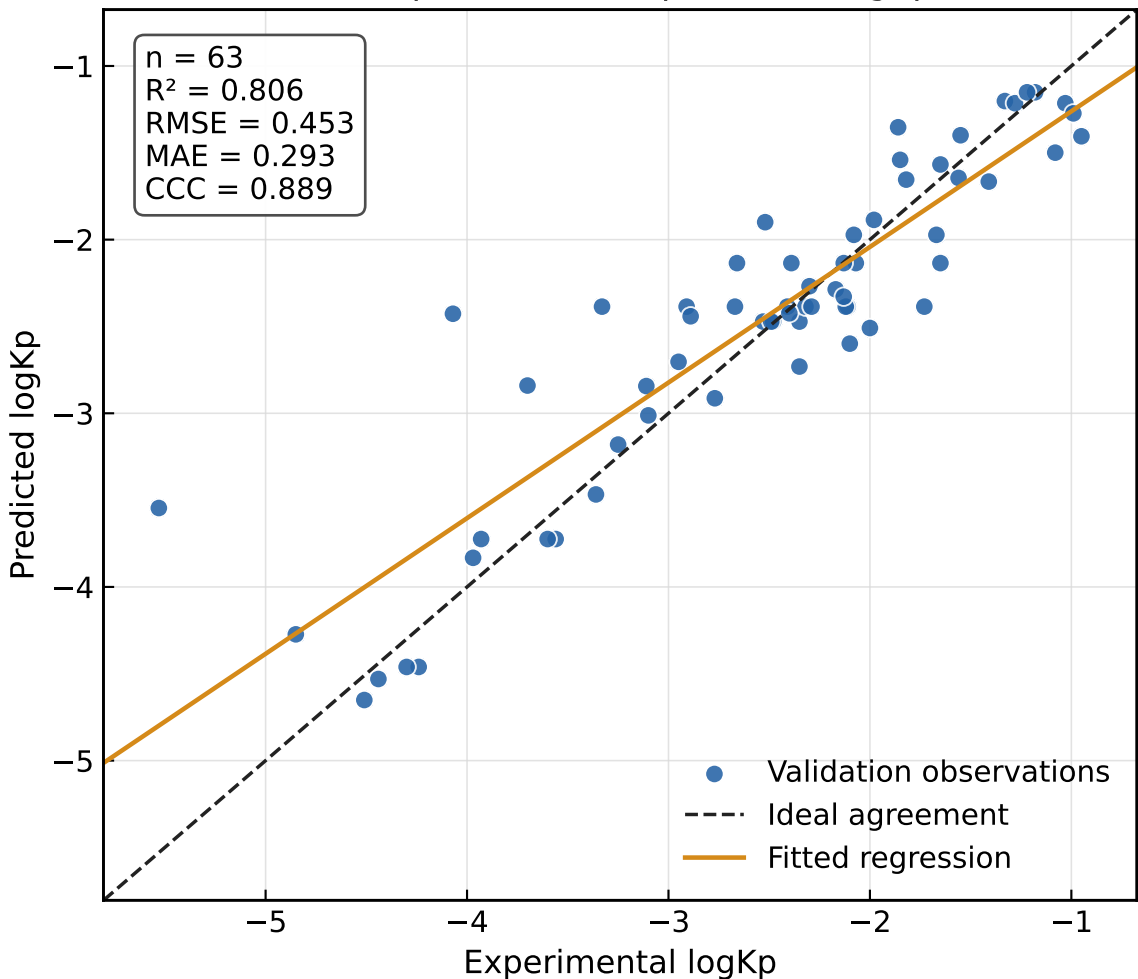
RF: experimental vs predicted logKp
