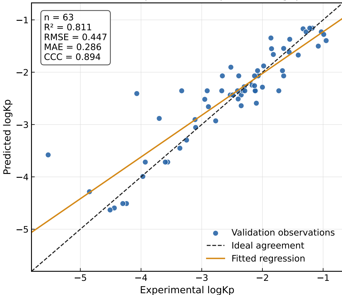
SVR (RBF): experimental vs predicted logKp
