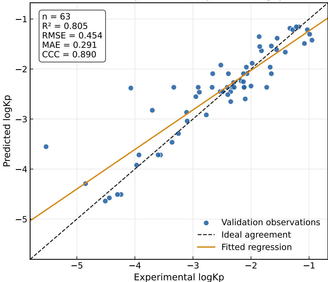
XGBoost: experimental vs predicted logKp
