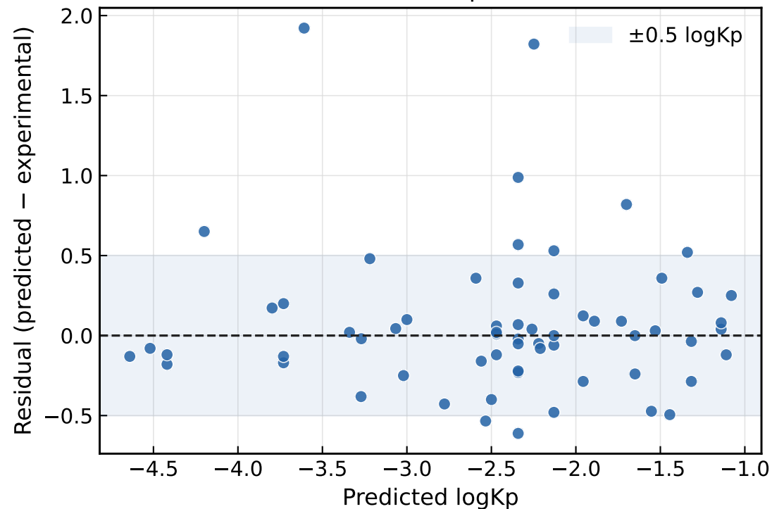
Residuals versus predictions
