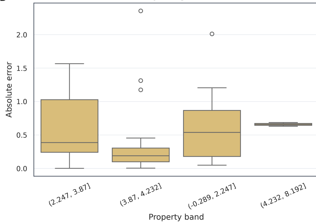
Error by XLogP quartile
