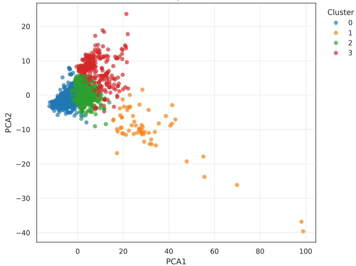
B External chemical-space clusters (k=4)
