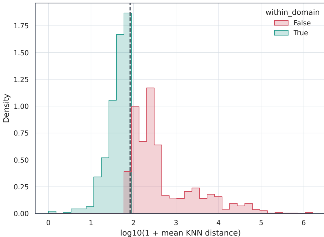
KNN applicability-domain distance
