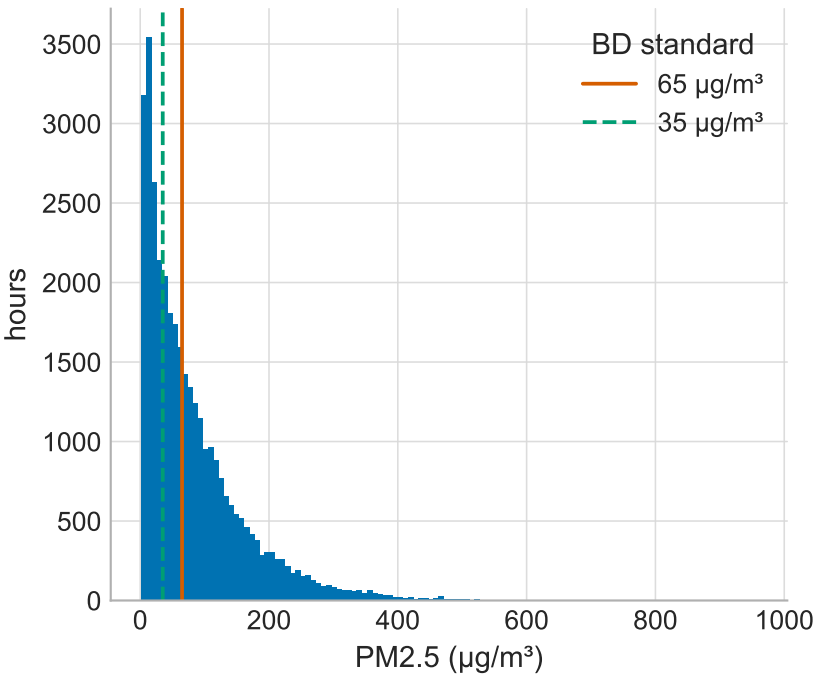
PM2.5 distribution, observed hours only distribution log1p distribution (modelling scale)
