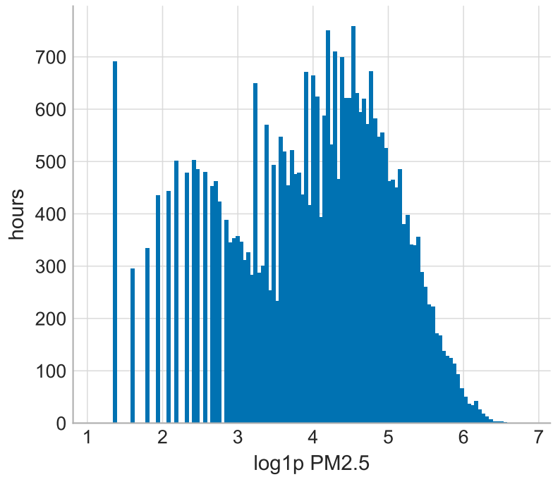
PM2.5 distribution, observed hours only distribution log1p distribution (modelling scale)
