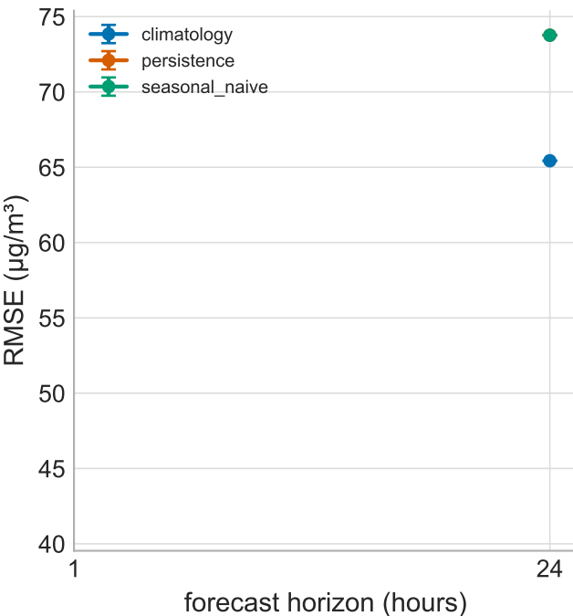
Tier 1 — baselines
