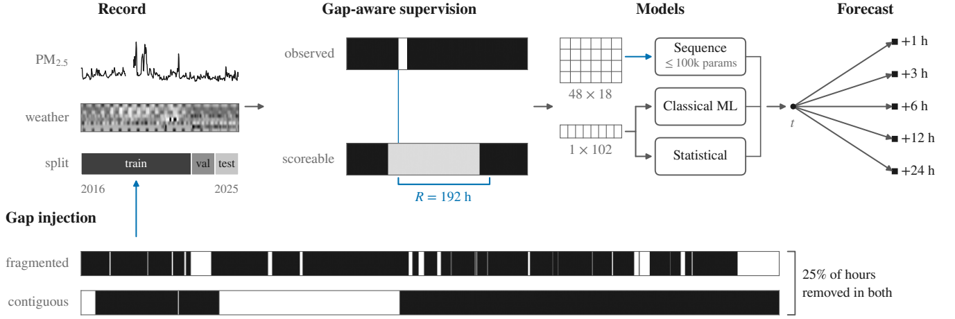
Fig. 1. Study design. A scored row requires unbroken history over a sterilisation radius R , drawn at the configured R = 192 h. Tabular models receive 102 engineered predictors per row; the sequence tier receives 18 contemporaneous channels over a window, because engineered history features restate what the window already contains. The lower panel shows the two injection arms, which remove the same number of observed hours and differ only in arrangement.
