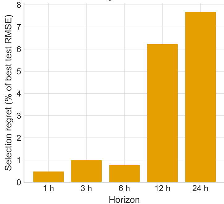
Cost of selecting on validation, not test
