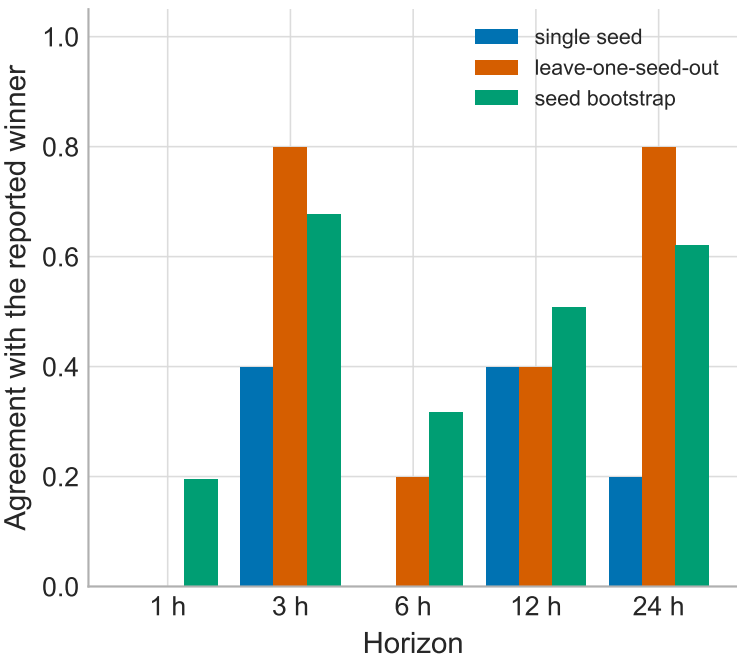
Does the winner survive resampling the seeds?
