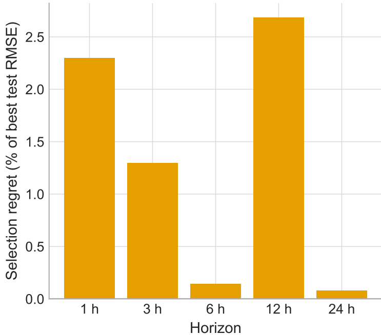
Cost of selecting on validation, not test
