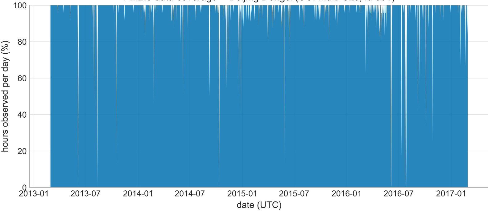
PM2.5 data coverage -- Beijing Dongsì (UCI Multi-Site, id 501)
