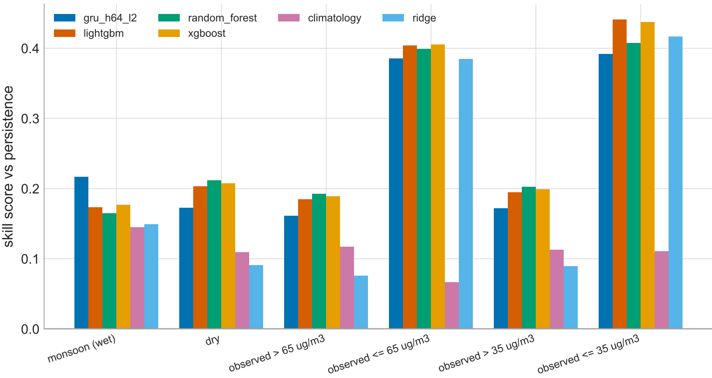
Skill by stratum at 24 hours (zero = no better than persistence)
