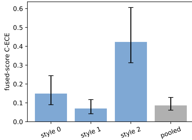
(b) with bootstrap CI
