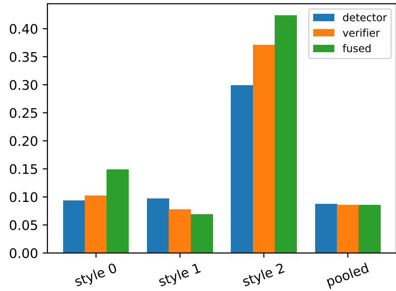
(c) stage decomposition
