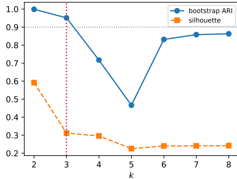
(a) cluster-count selection
