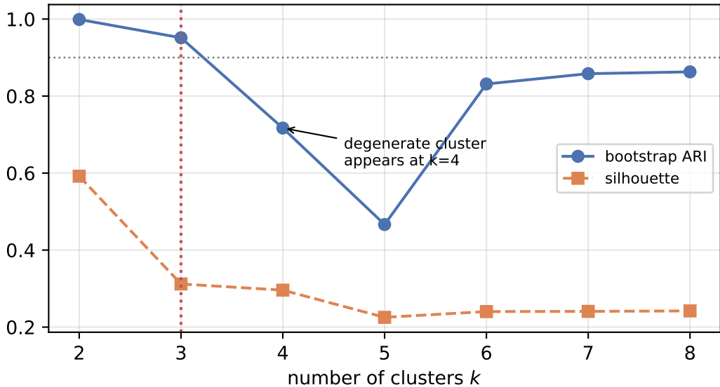
Visual-style cluster count
