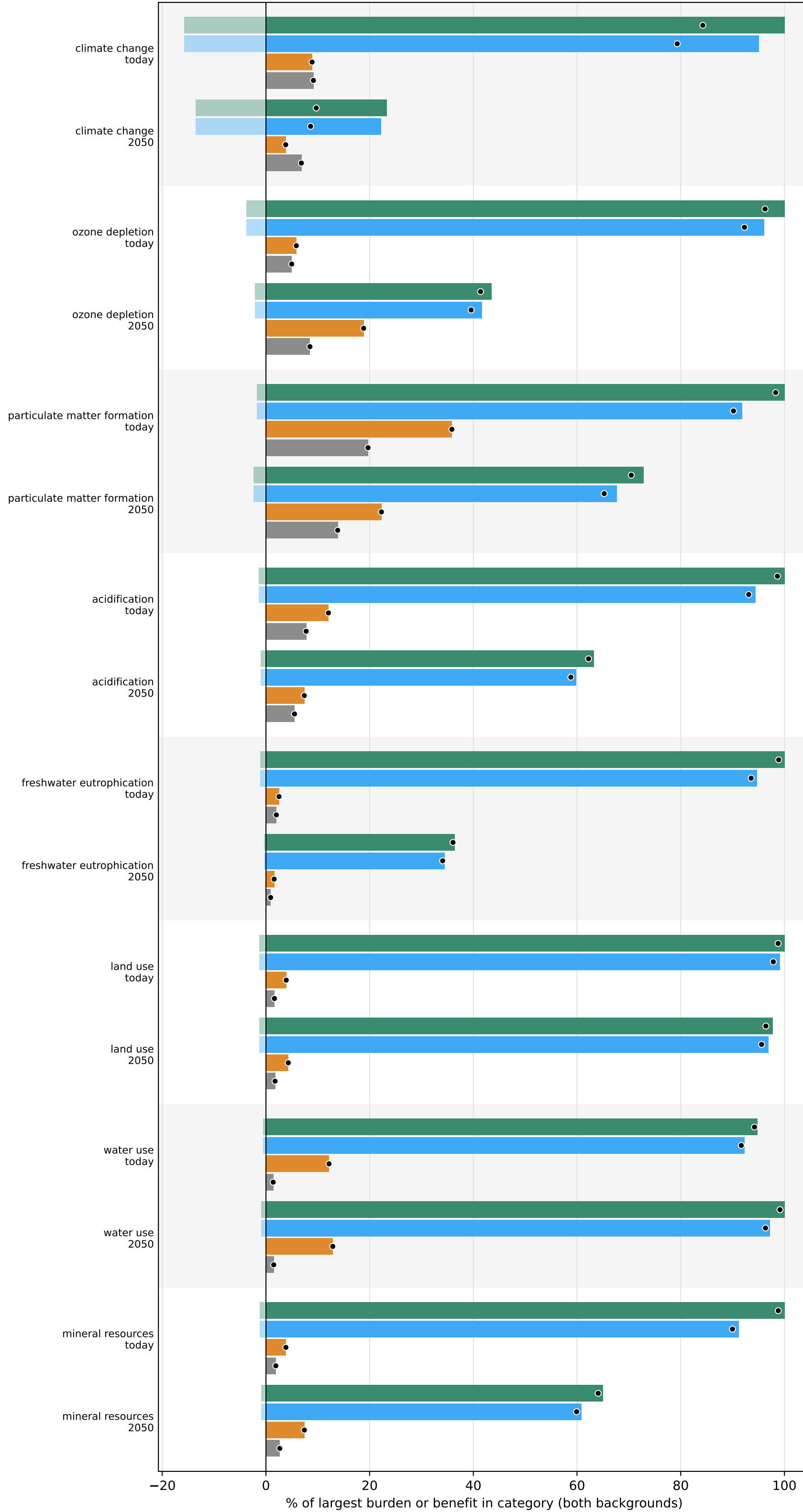
RAW biopol (3D-printed wall): today vs. 2050 wall length = 4 m, reference service life 50 yr
