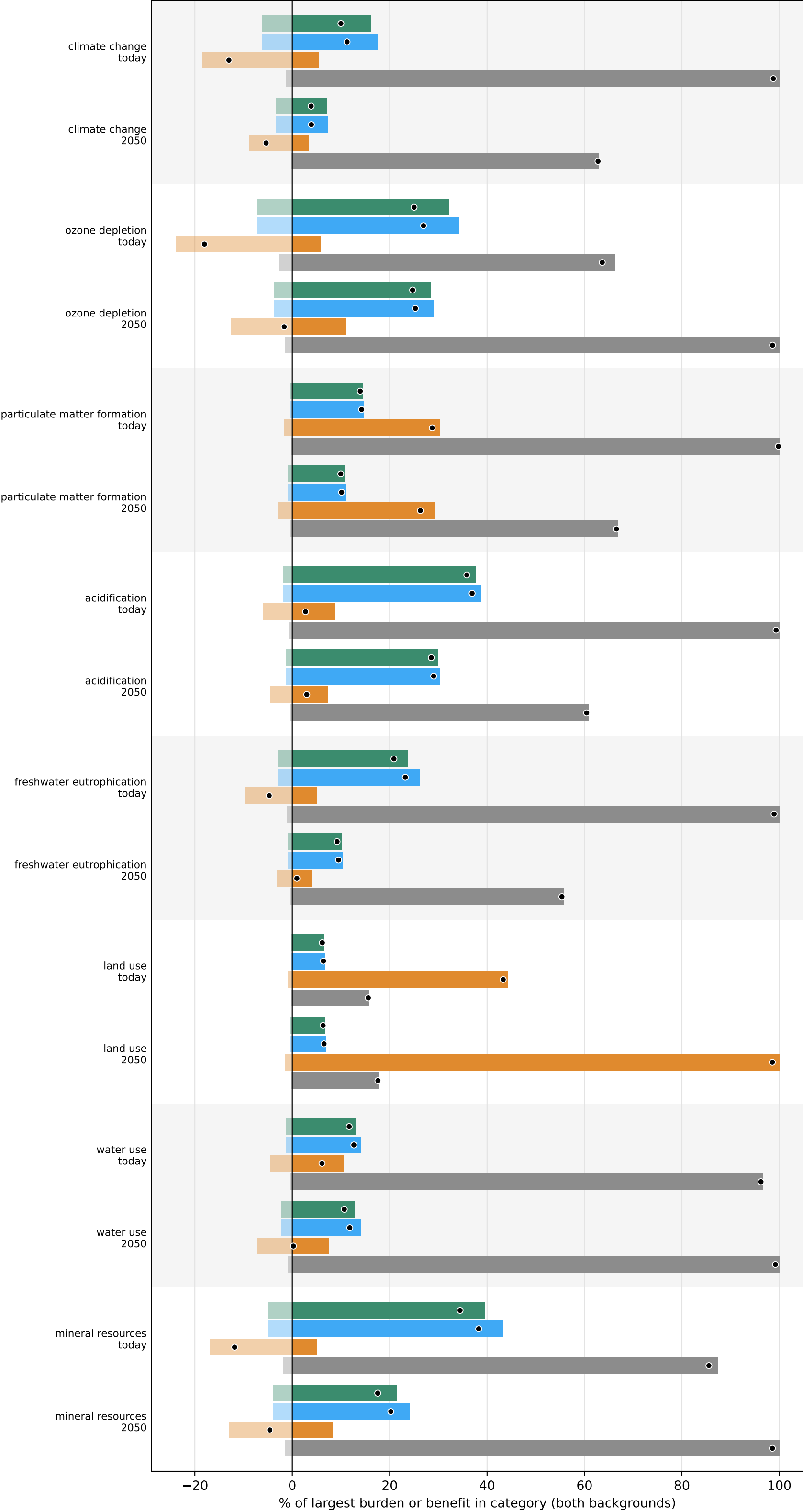
RAW coreless filament winding (beam): today vs. 2050 beam span = 6 m, reference service life 50 yr
