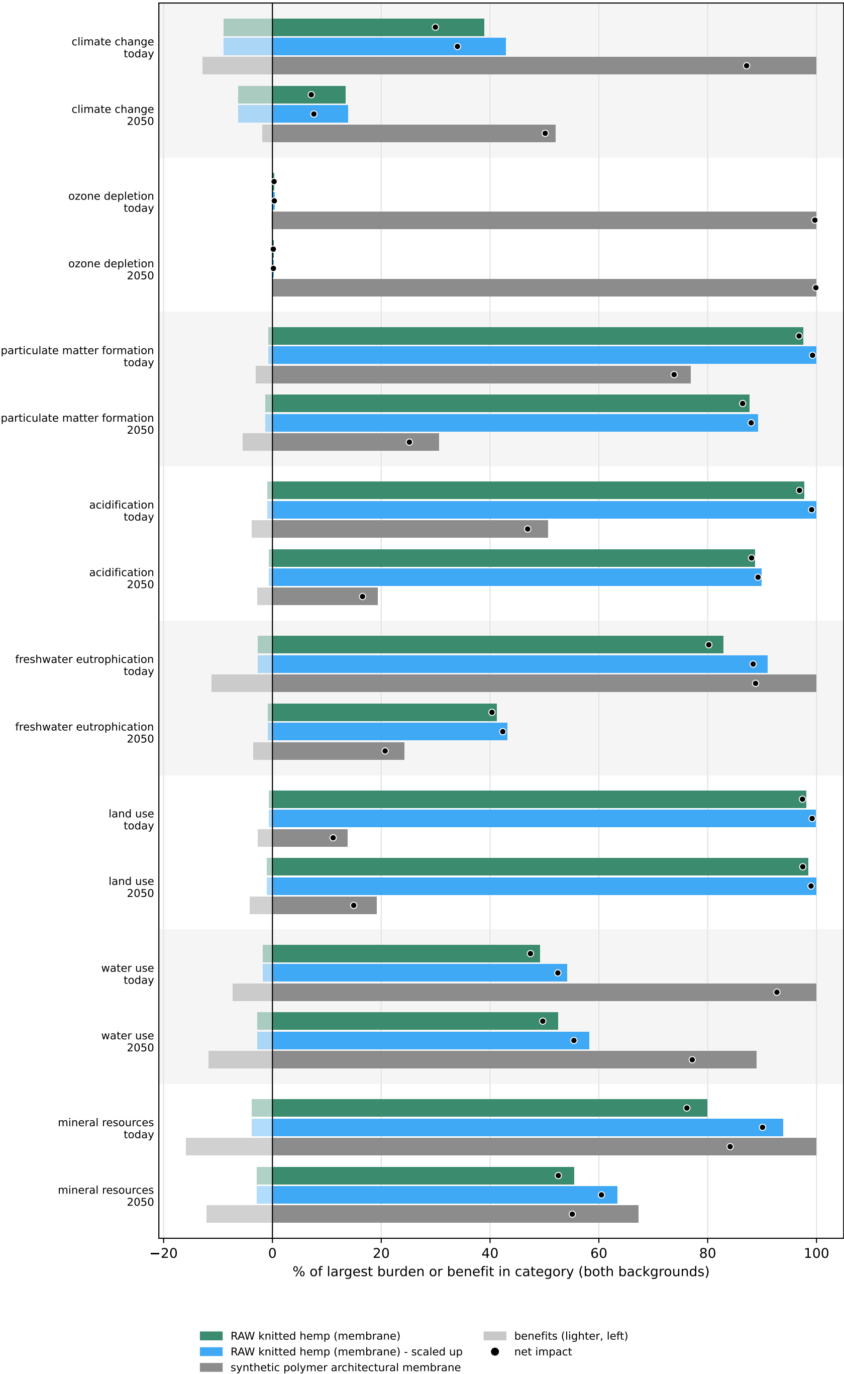
RAW knitted hemp (membrane): today vs. 2050 membrane coverage = 100 m2, reference service life 50 yr
