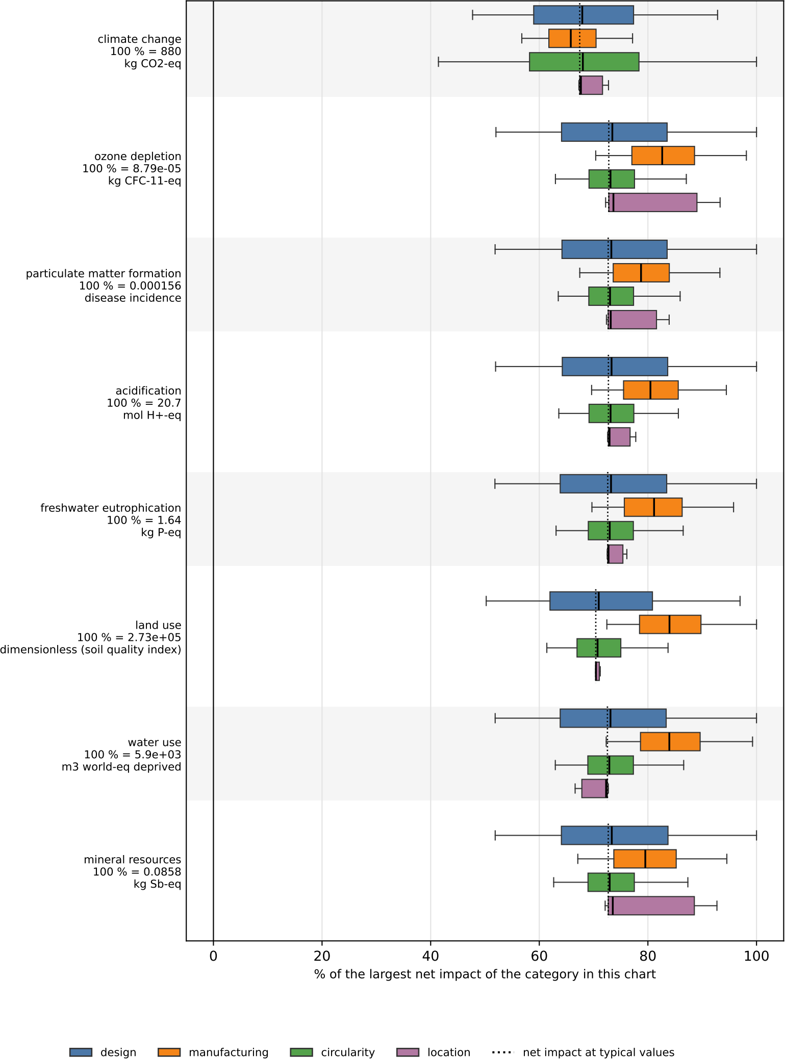
RAW biopol (3D-printed wall) (2050) range of the net impact when one parameter group is varied (2000 draws)
