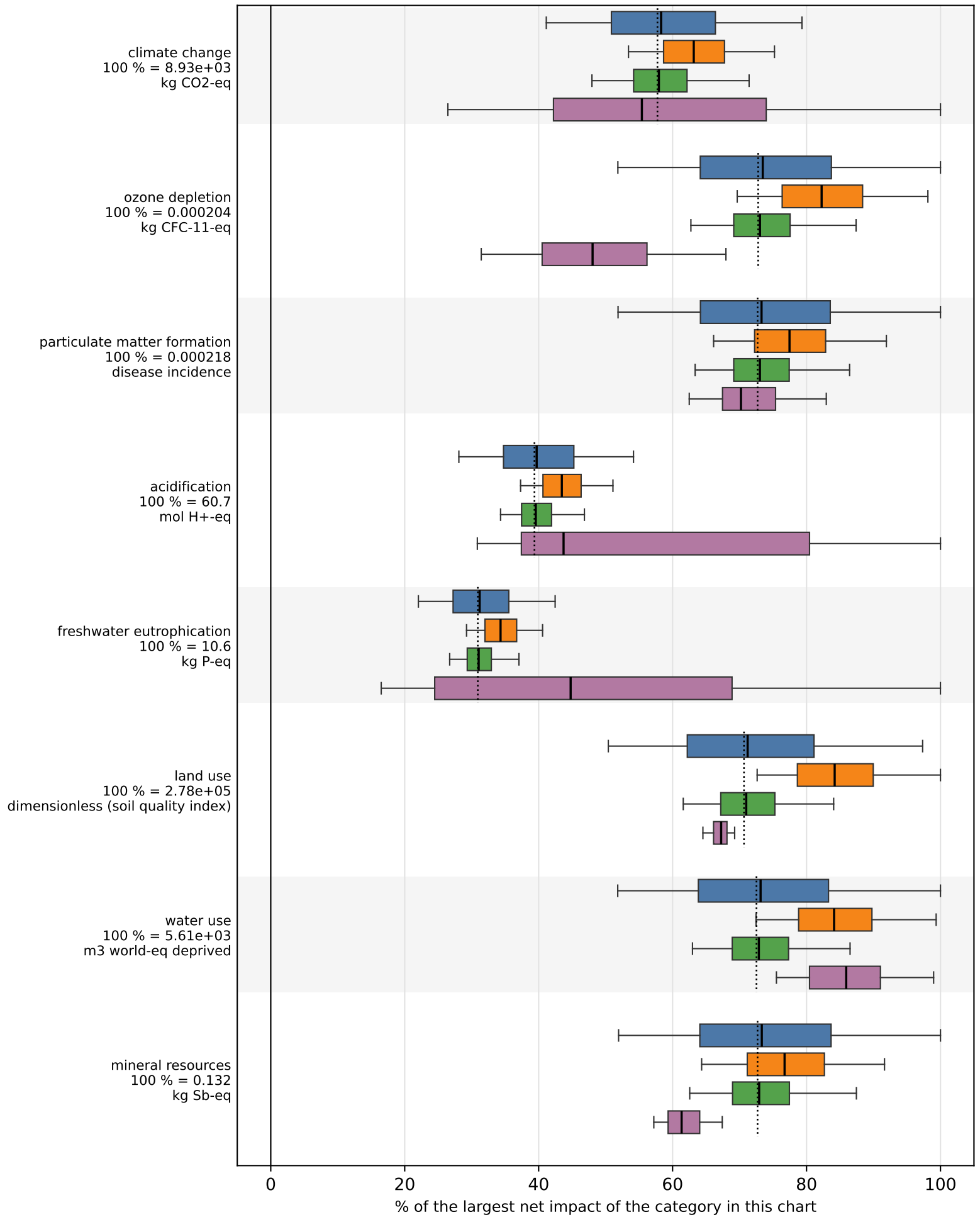
RAW biopol (3D-printed wall) (today) range of the net impact when one parameter group is varied (2000 draws)
