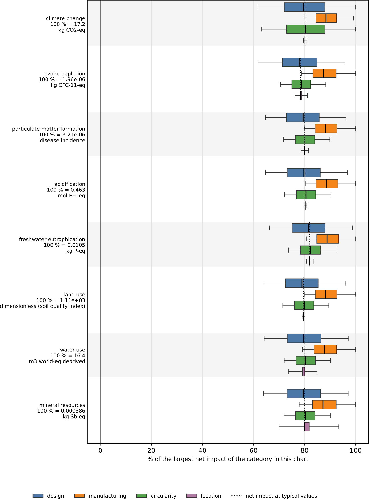
RAW coreless filament winding (beam) (2050) range of the net impact when one parameter group is varied (2000 draws)
