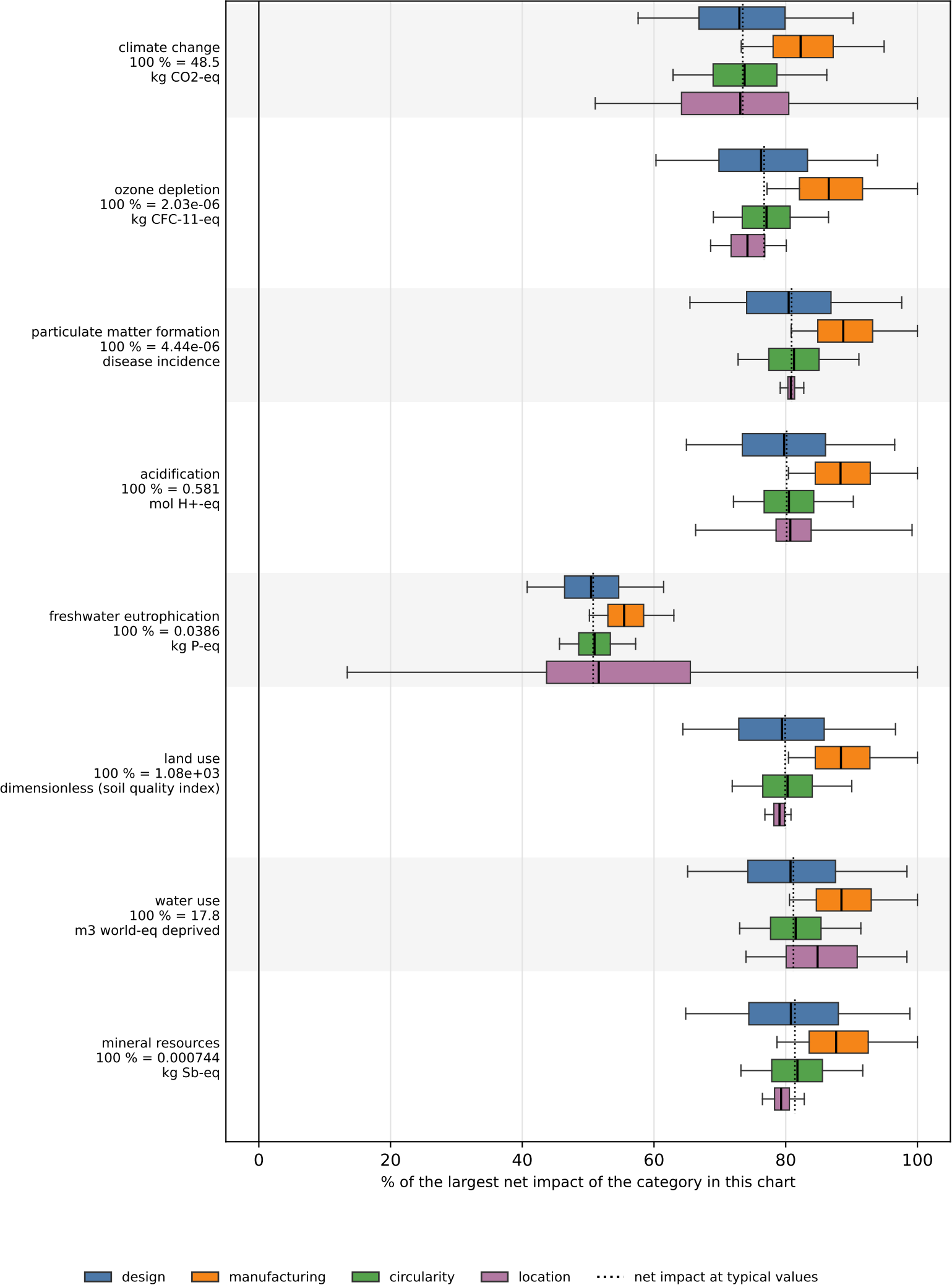
RAW coreless filament winding (beam) (today) range of the net impact when one parameter group is varied (2000 draws)
