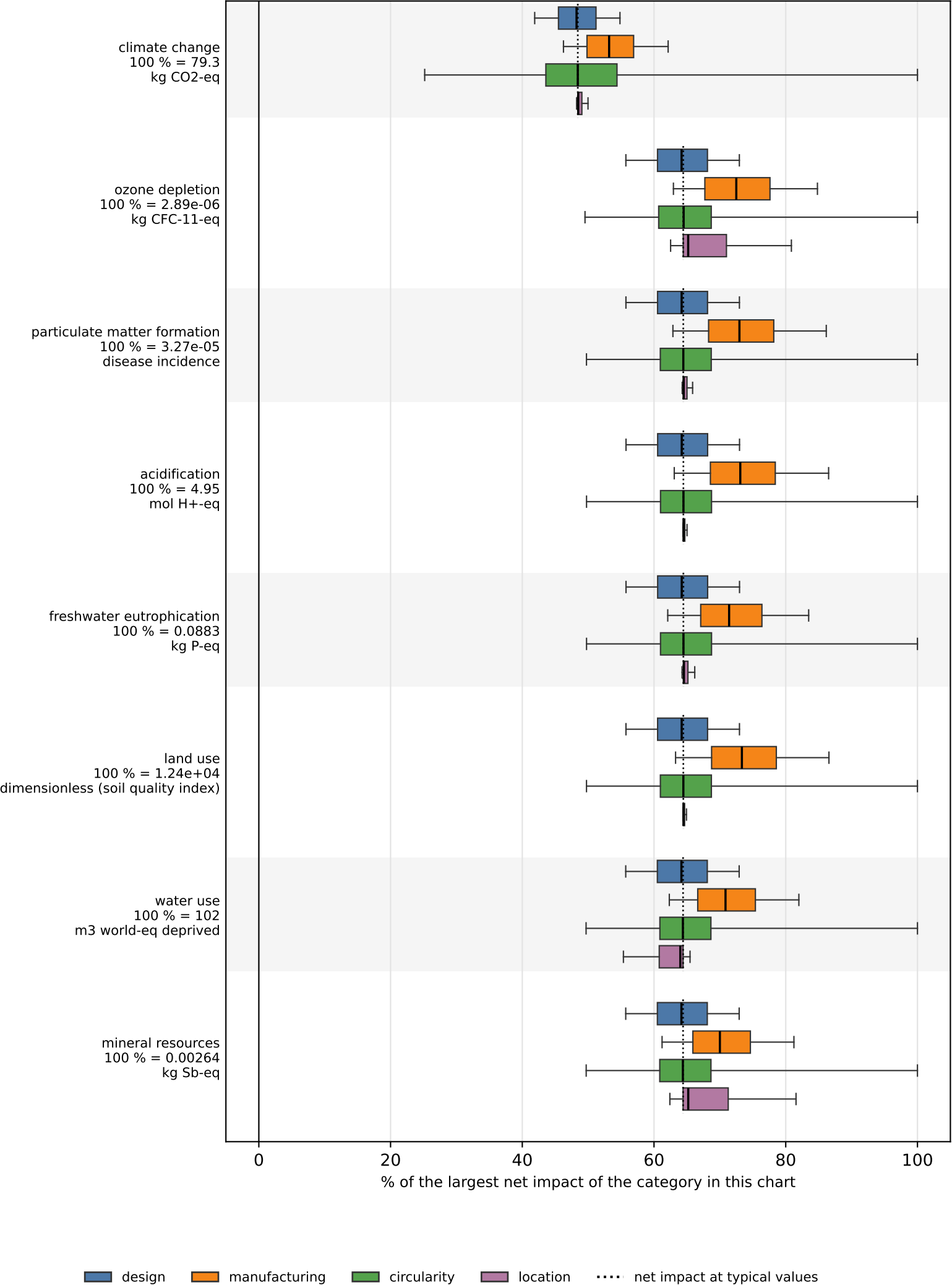
RAW knitted hemp (membrane) (2050) range of the net impact when one parameter group is varied (2000 draws)
