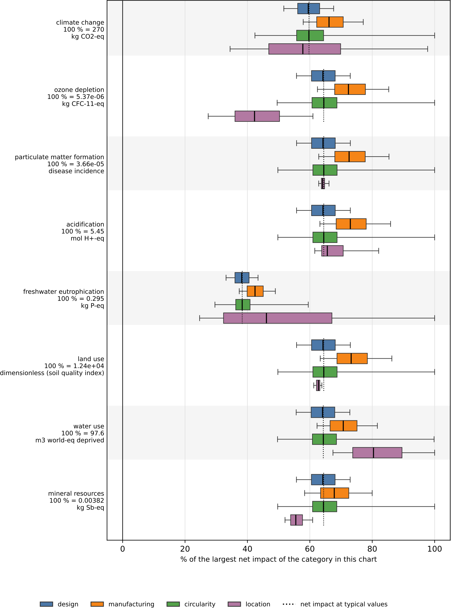
RAW knitted hemp (membrane) (today) range of the net impact when one parameter group is varied (2000 draws)
