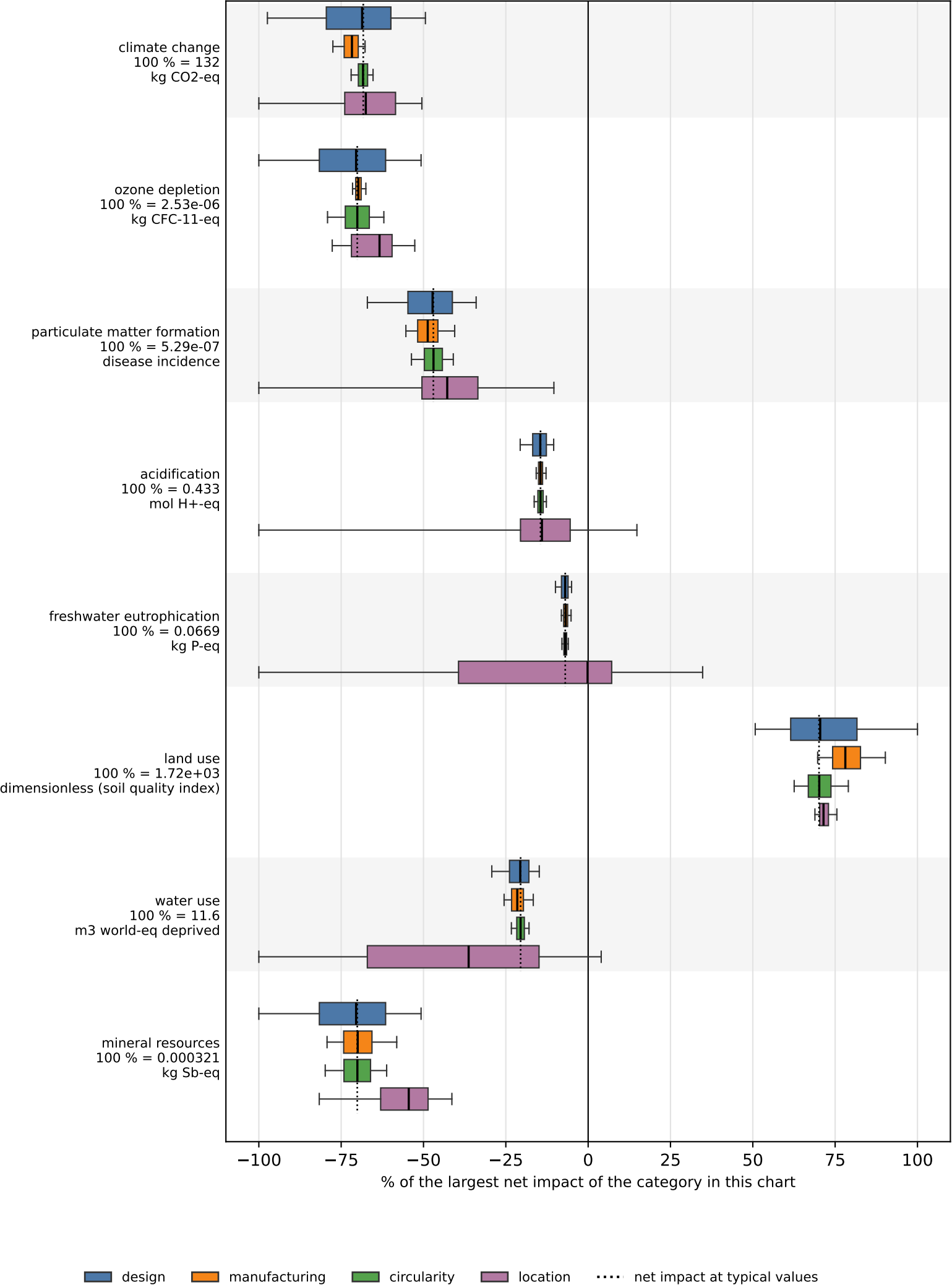
RAW reclaimed timber (CNC beam) (today) range of the net impact when one parameter group is varied (2000 draws)
