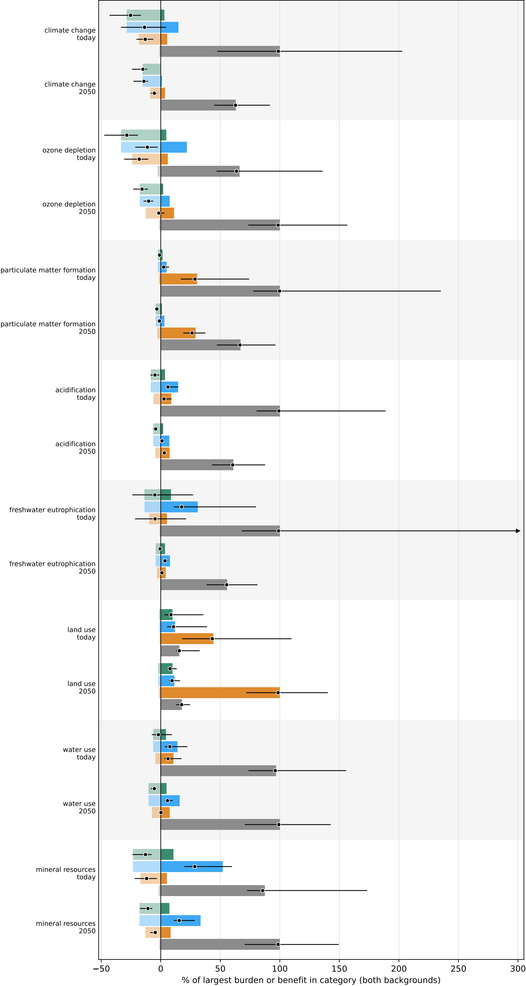
RAW reclaimed timber (CNC beam): today vs. 2050, with 5-95 % intervals beam span = 6 m, 2000 draws
