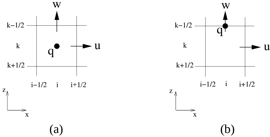
Figure 5.2: Applied arrangements of the unknowns in a staggered grid: (a) standard layout and (b) box layout. Meaning of the unknowns: u is the horizontal velocity, w is the vertical velocity and q is the non-hydrostatic pressure.
