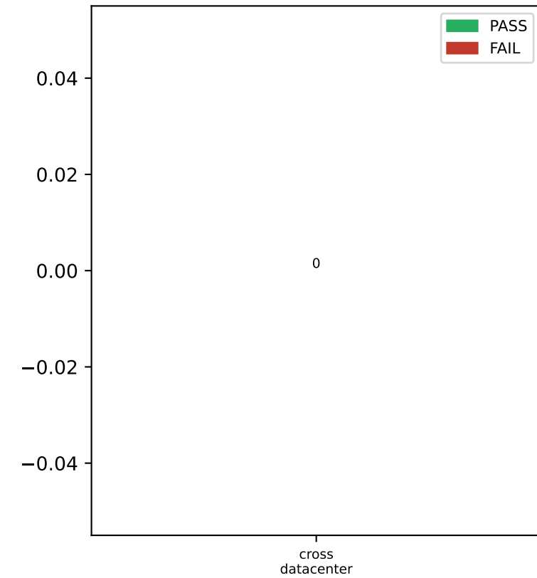
Leader Elections
