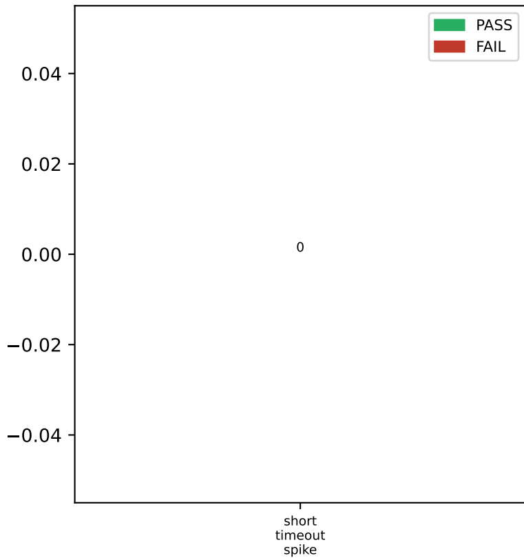
Leader Elections
