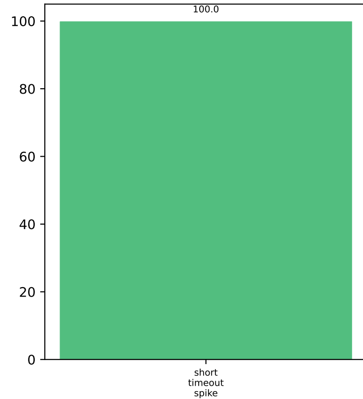
Success Rate (%)
