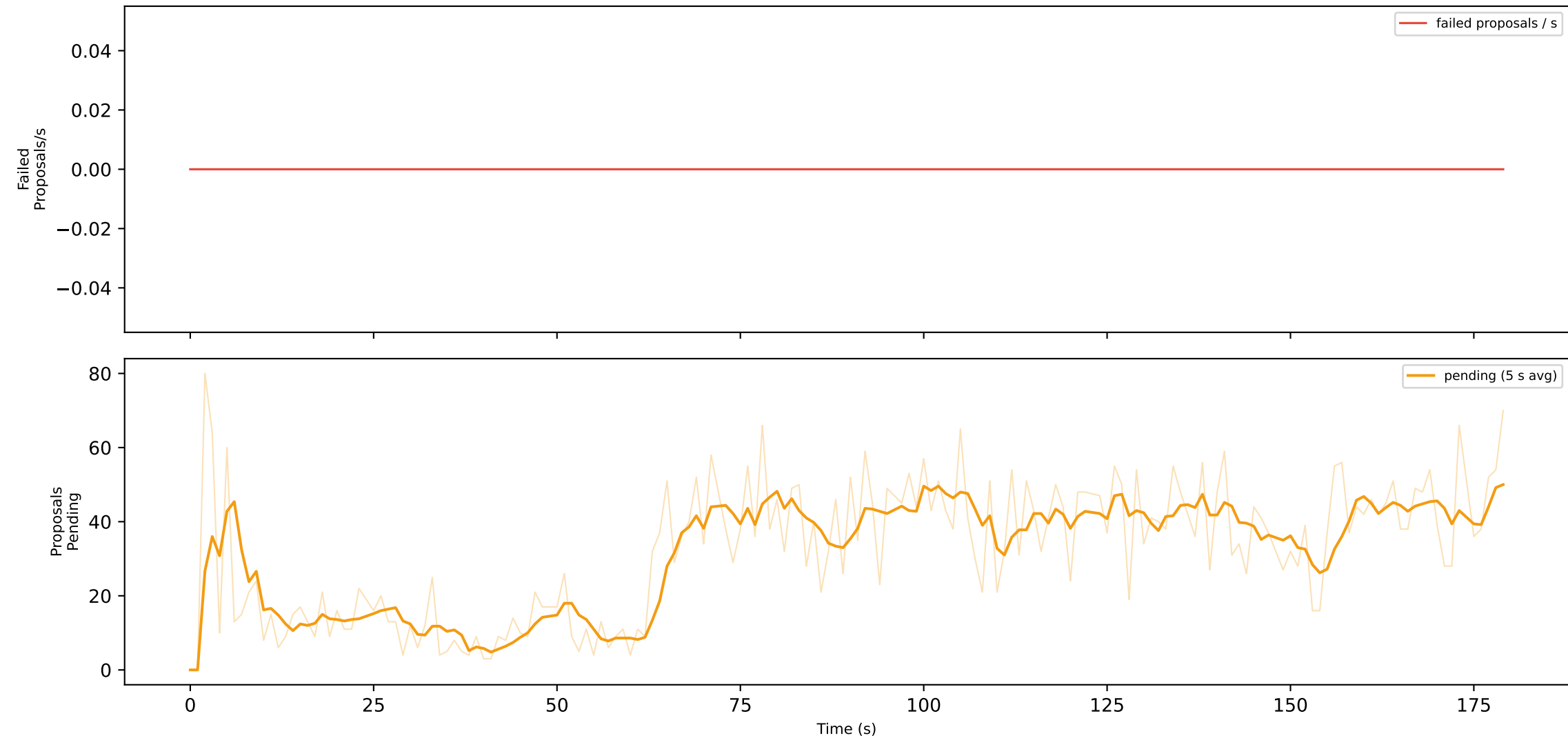
sustained_write_flood - supporting metrics
