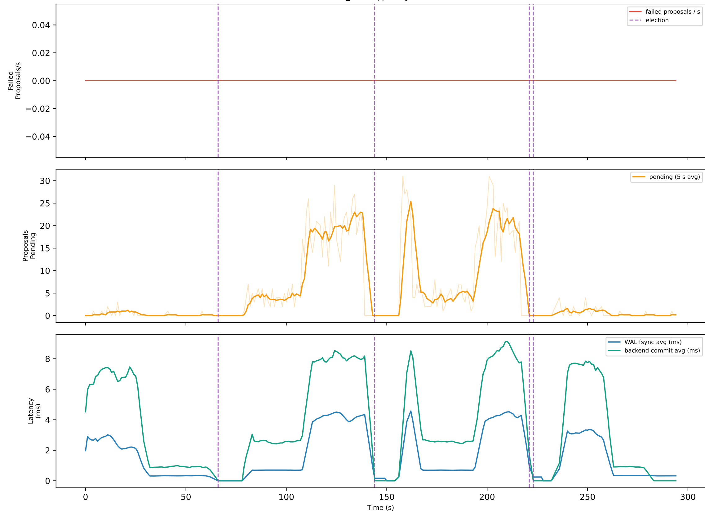
leader_kill - supporting metrics
