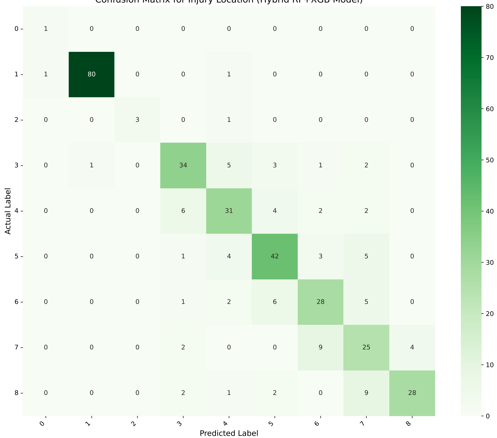
Confusion Matrix for Injury Location(Hybrid RF+XGB Model)
