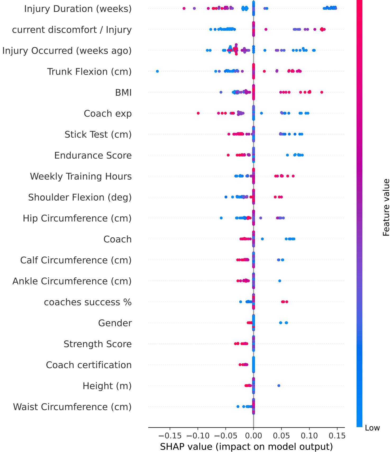
SHAP Summary Plot for "Severe" Injury Risk (Hybrid4)
