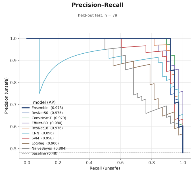
(b) Precision-recall curves.
