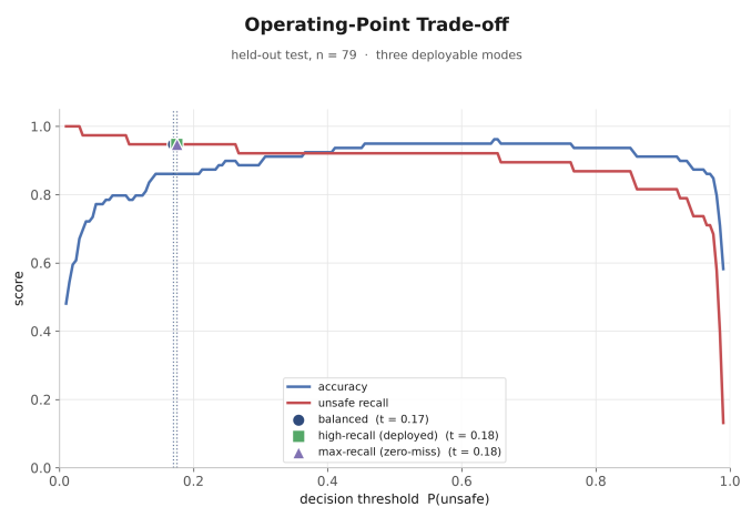
Fig. 12. Ensemble threshold selection on the held-out test set: accuracy and unsafe recall against the decision threshold, with the balanced, high-recall, and max-recall operating points marked. Because the retrained dataset is near-balanced, the three points nearly coincide.
