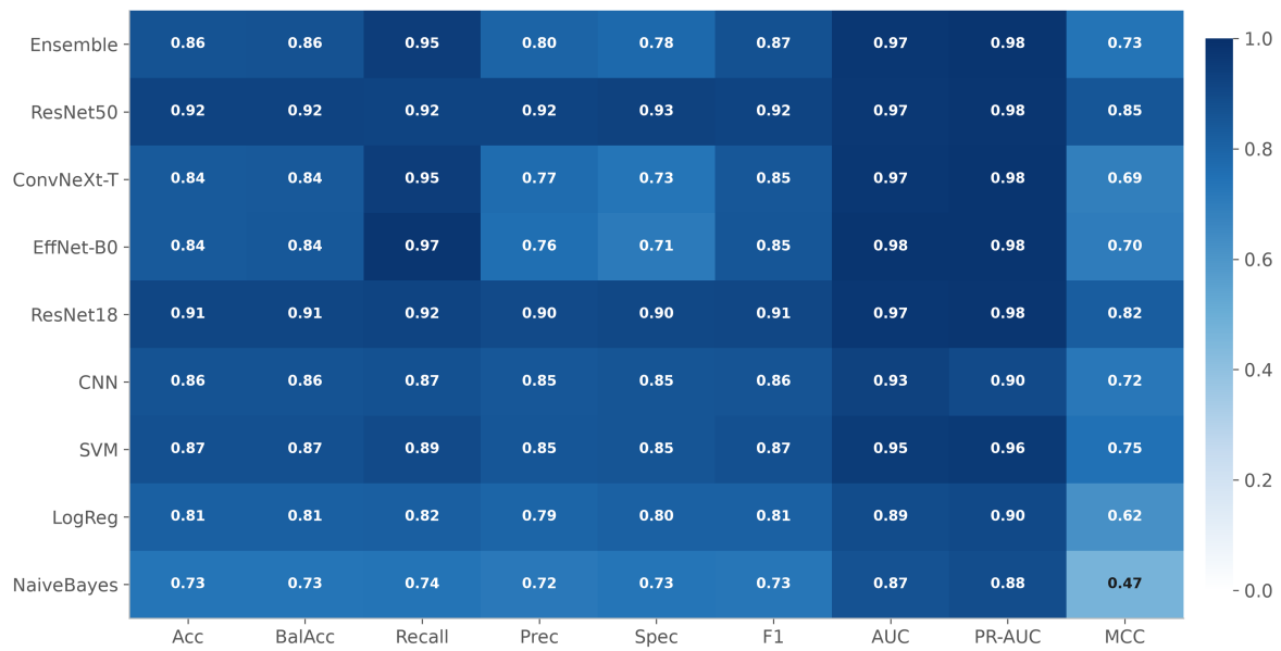
Fig. 9. Heatmap of held-out test metrics for all nine models at the balanced operating point.
