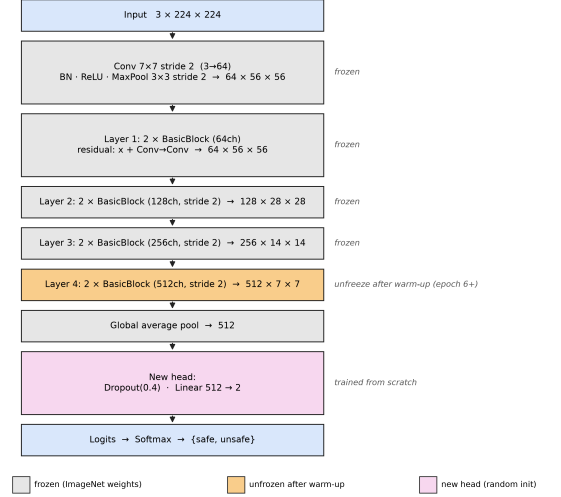
Fig. 7. Two-phase transfer-learning scheme, illustrated with ResNet18. The ImageNet-pretrained backbone is frozen during a short head-only warm-up, its deepest stage is then unfrozen for fine-tuning, and a new classifier head is trained from scratch. ResNet50, EfficientNet-B0, and ConvNeXt-Tiny follow the same procedure at a 224 \times 224 input resolution.
