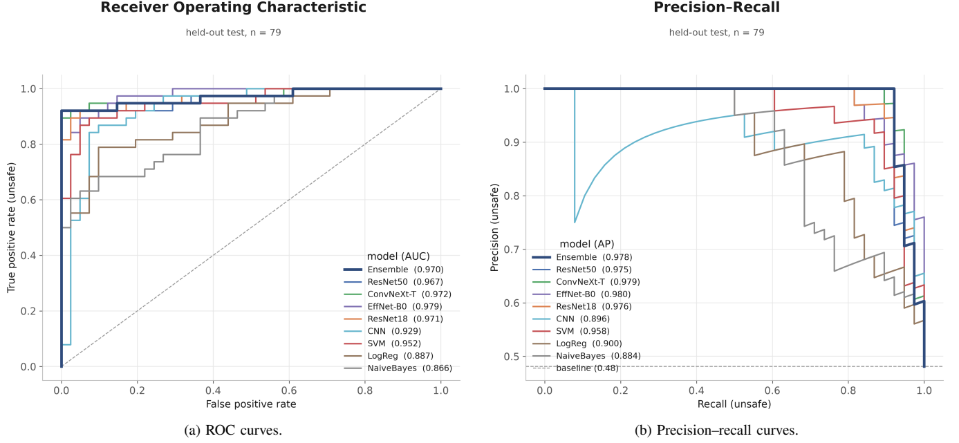
Fig. 9. Receiver operating characteristic and precision-recall curves for all nine models on the held-out test set.
