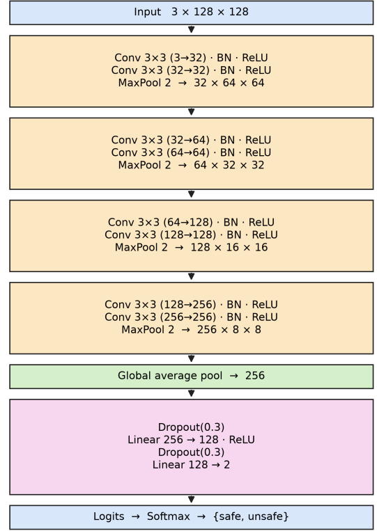
Fig. 6. Scratch CNN architecture used for image-level binary classification.
