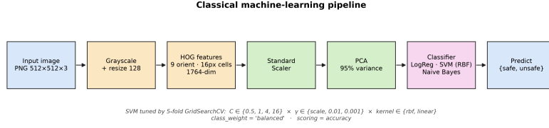
Figure 5: Overview of the HOG-based classical machine-learning pipeline.
