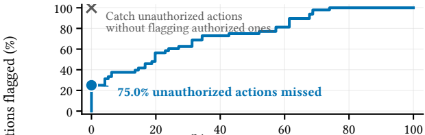
(b) Gemma scorer
