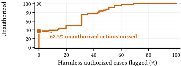
(b) Gemma scorer
