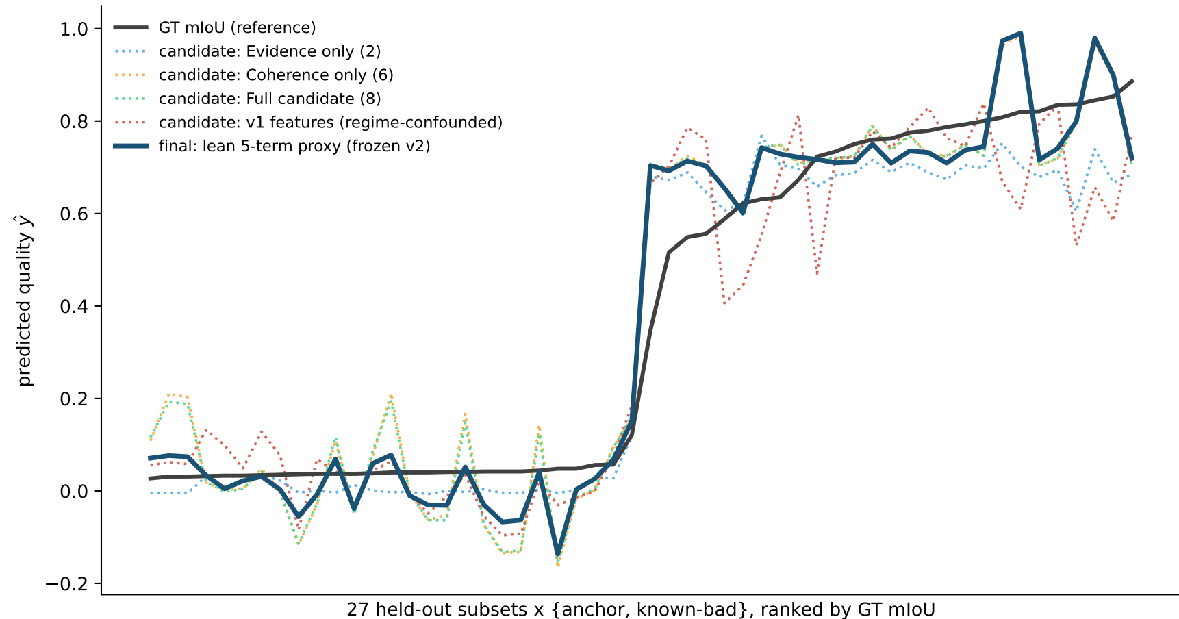
Candidate proxies explored during training vs the final frozen proxy (all fitted on the same anchor-trial table; evaluated on unseen holdouts)
