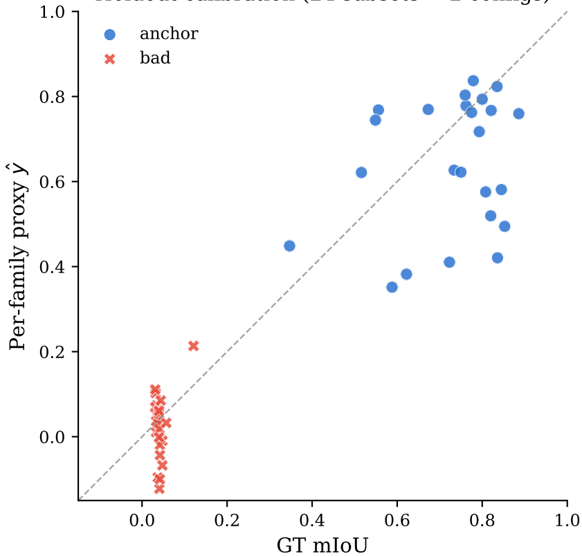
Holdout calibration (24 subsets \times 2 configs)
