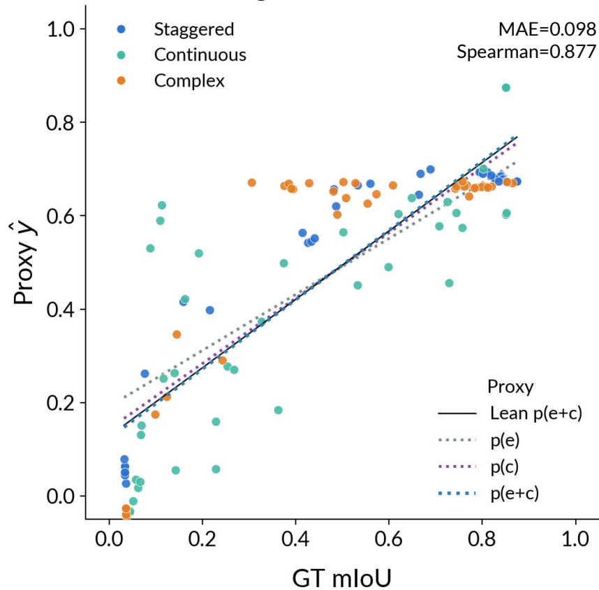
Training: 40 trials \times 3 anchors
